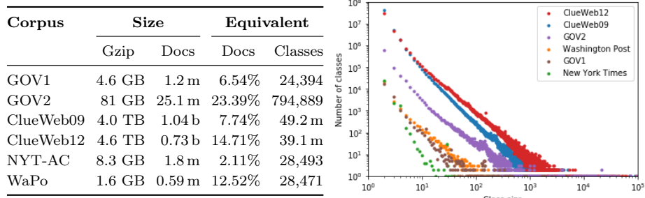
Fig. 1. Overview of the studied corpora (left), and the size of equivalence classes (right).
