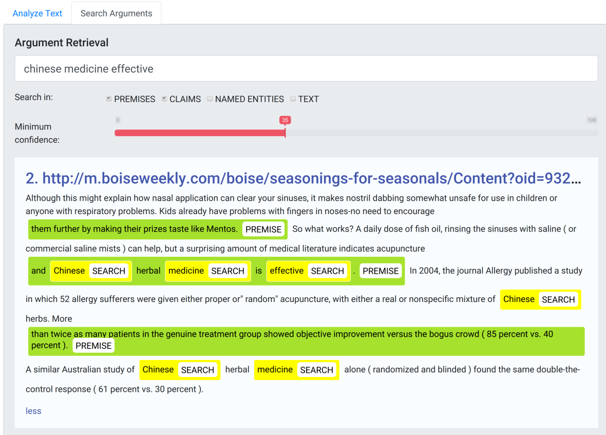
Figure 3: Search Arguments: query box, field selectors, and result with link to the original document.
