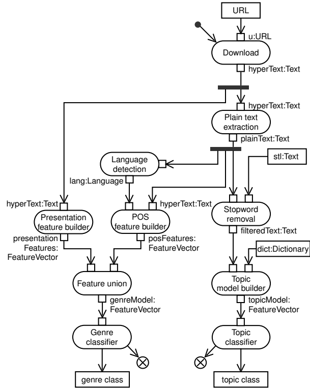
Figure 2. IR process for the sample categorization task, specified as UML activity diagram.
